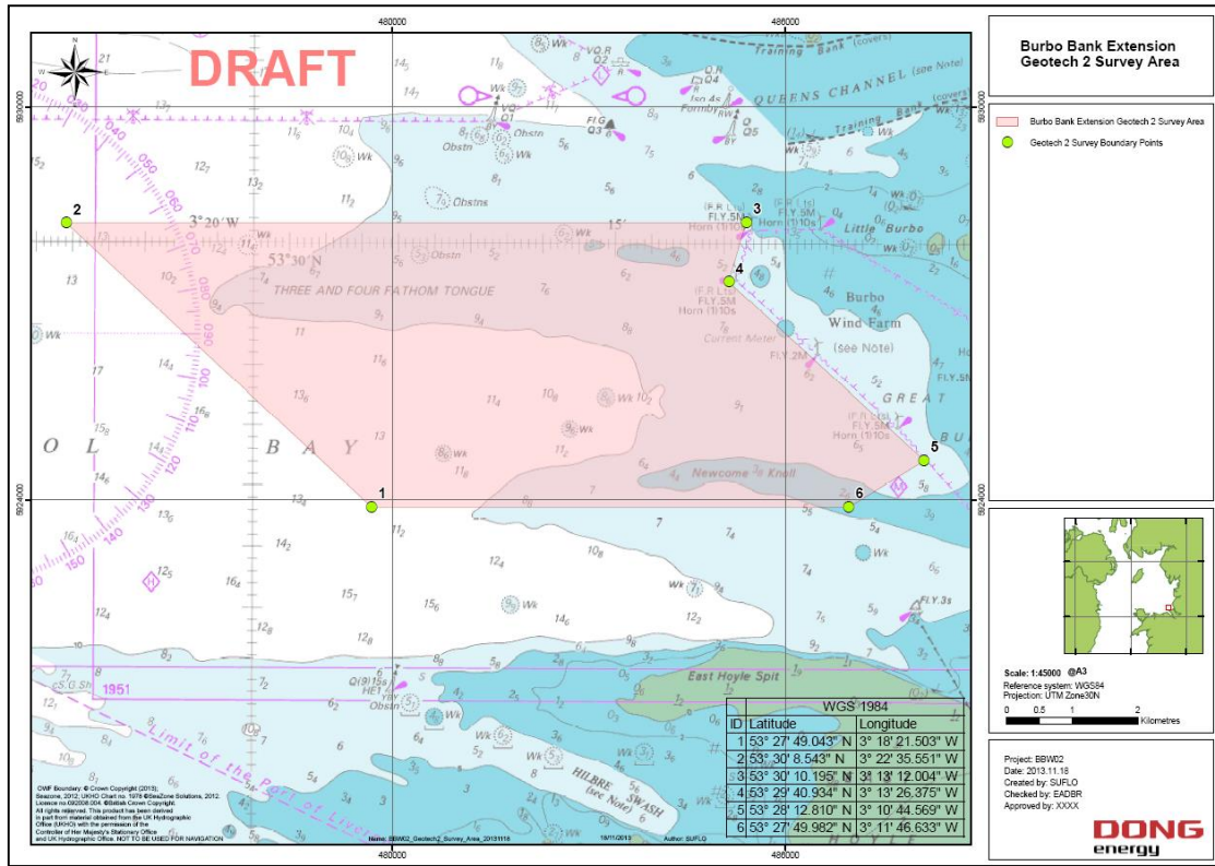
SURVEY AREA SHADED WITH CORNER CO-ORDINATES MARKED
