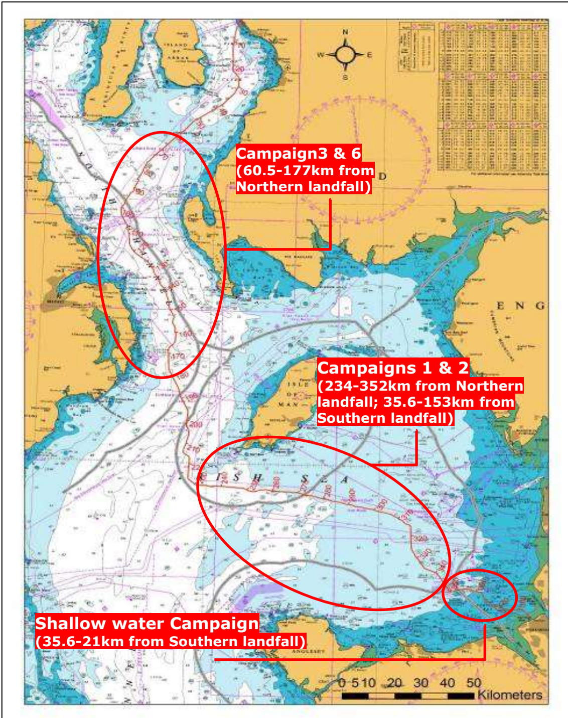
Figure 1 – Western Link cable route - Installation campaigns
