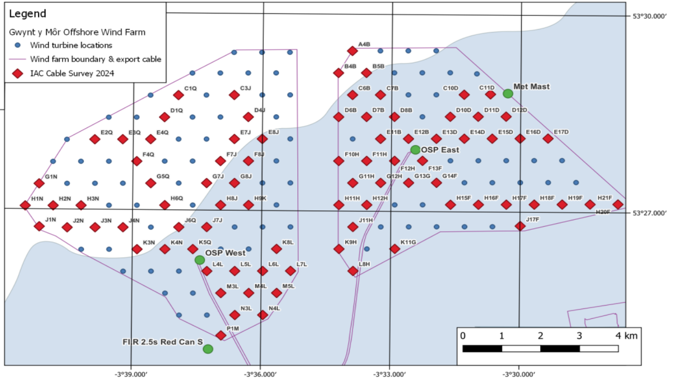
Figure 1: IAC Cable Survey 2024, image credit: AWJ Marine
